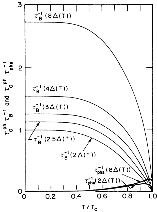
FIG. 15. Phonon pair-breaking rate \tau_B^{-1}(\Omega, T) in units of (\tau_0^{ph})^{-1} and the phonon scattering rate \tau_{ph}^{-1}(\Omega, T) in units of (\tau_0^{ph})^{-1} , vs T/T_c . The phonon energies \Omega in this plot are multiples of the gap energy \Delta(T) . \tau_0^{ph} for various materials is given in Table II.
