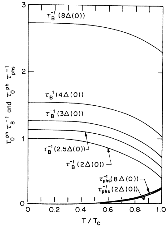
FIG. 16. Phonon pair-breaking rate \tau_B^{-1}(\Omega, T) in units of (\tau_0^{ph})^{-1} and the phonon scattering rate \tau_{ph}^{-1}(\Omega, T) in units of (\tau_0^{ph})^{-1} , vs T/T_c . The phonon energies \Omega are constants in this plot. \tau_0^{ph} for various materials is given in Table II.
