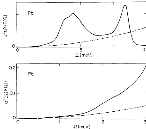
FIG. 5. Plot of \alpha^2(\Omega)F(\Omega) (solid) and b\Omega (dashed) vs \Omega for Pb. The lower part shows an enlargement of the low-frequency region.
